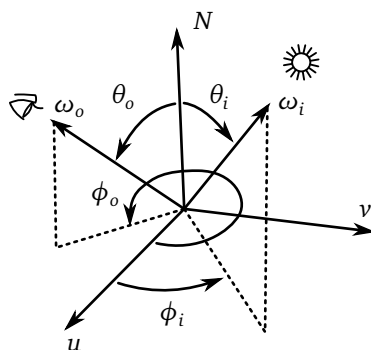
Figure 5.3: Geometry for local surface reflection.
