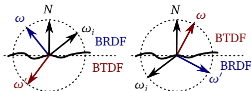
Figure 5.4: The bidirectional (surface) scattering distribution (BSDF) implicitly defines two reflectance and transmittance distributions (BRDFs and BTDFs), depending on which side of the hemisphere around surface normal N the incident direction \omega_i is located. This greatly simplifies handling materials that both reflect and transmit light, which—due to the Fresnel effect—is quite common in transparent and translucent objects.
