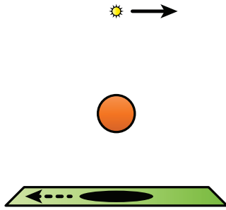
Figure 7.4: Direct vs. indirect manipulation of a point light source. With direct manipulation, the user moves the light source (solid arrow) and the shadow follows accordingly (dashed arrow). Direct interfaces are trivial to implement, but quickly become counter-intuitive in complex scenes. With indirect/goal-based manipulation, the user moves/sketches the shadow (dashed arrow) and the system solves for the new light source position (solid arrow). Image taken from [202].
