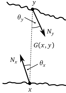
Figure 2.2: The geometry term G(x, y) accounts for the relative distance and orientation of two surface points x and y .
