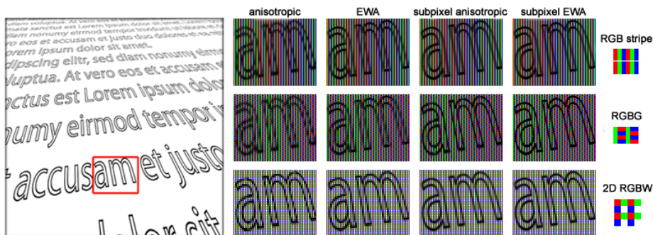
Figure 4.1: Subpixel rendering of a plane with a structured texture for different subpixel layouts, similar to those found in diverse displays nowadays. This image showcases high-quality texture filtering, one of the applications of our proposed optimal filtering framework, comparing standard filtering (anisotropic and EWA) to our subpixel-aware filtering (again, using anisotropic and EWA). Note how our method significantly reduces aliasing. Image taken from [47].
