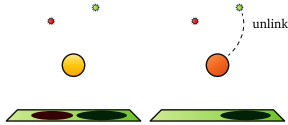
Figure 7.6: Light linking. Left: Original configuration with two colored point light sources and two objects (a sphere and a ground plane). Right: The green point light source (upper right) is unlinked from the sphere object, hence also casting no shadow onto the bottom plane anymore. Image taken from [202].
